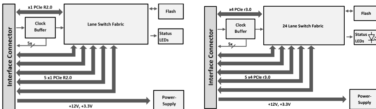
Figure 5: PCIe 6 Lane Switch Module Gen2
