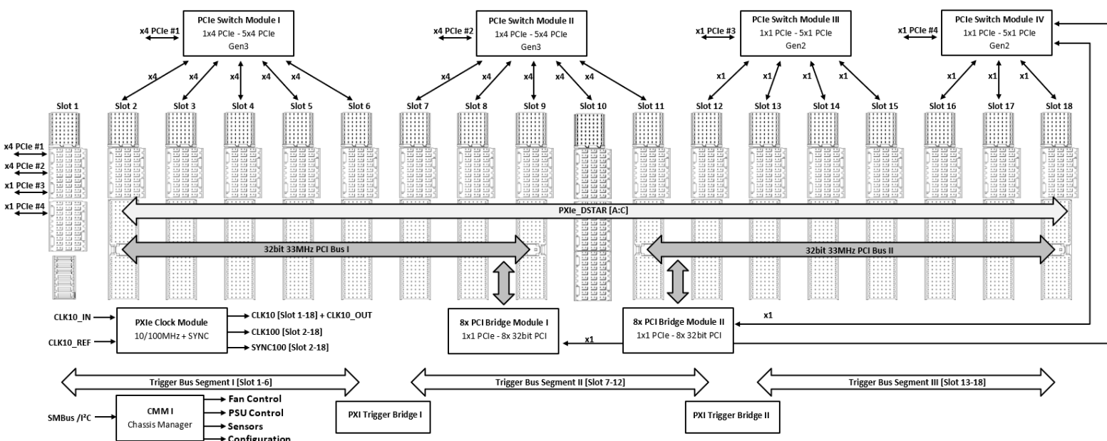
Figure 3: Backplane Topology
